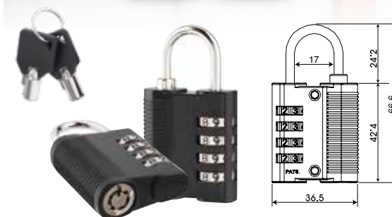
PL570 Window Dial™ Shackle size: Ø3.8 mm W36.5 x D16 x H66.6 mm
