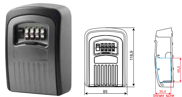
PL967 W85 x D35.9 x H118.9 mm Inner size: W64.7 x D30.4 x H48.5 mm
