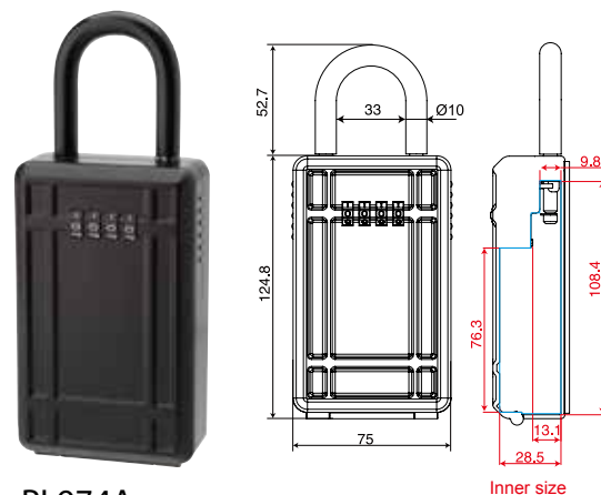
PL974A Shackle size: Ø10 mm W75 x D33.35 x H177.5 mm Inner size: W71.2 x D28.5 x H108.4 mm
